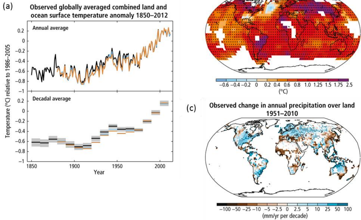
Figure 2: (a) Observed globally averaged combined land and ocean surface temperature anomalies (relative to the mean of 1986 to 2005 period, as annual and decadal averages); (b) Map of the observed surface temperature change, from 1901 to 2012; (c) Map of observed precipitation change, from 1951 to 2010 (Source: IPCC 2014).
